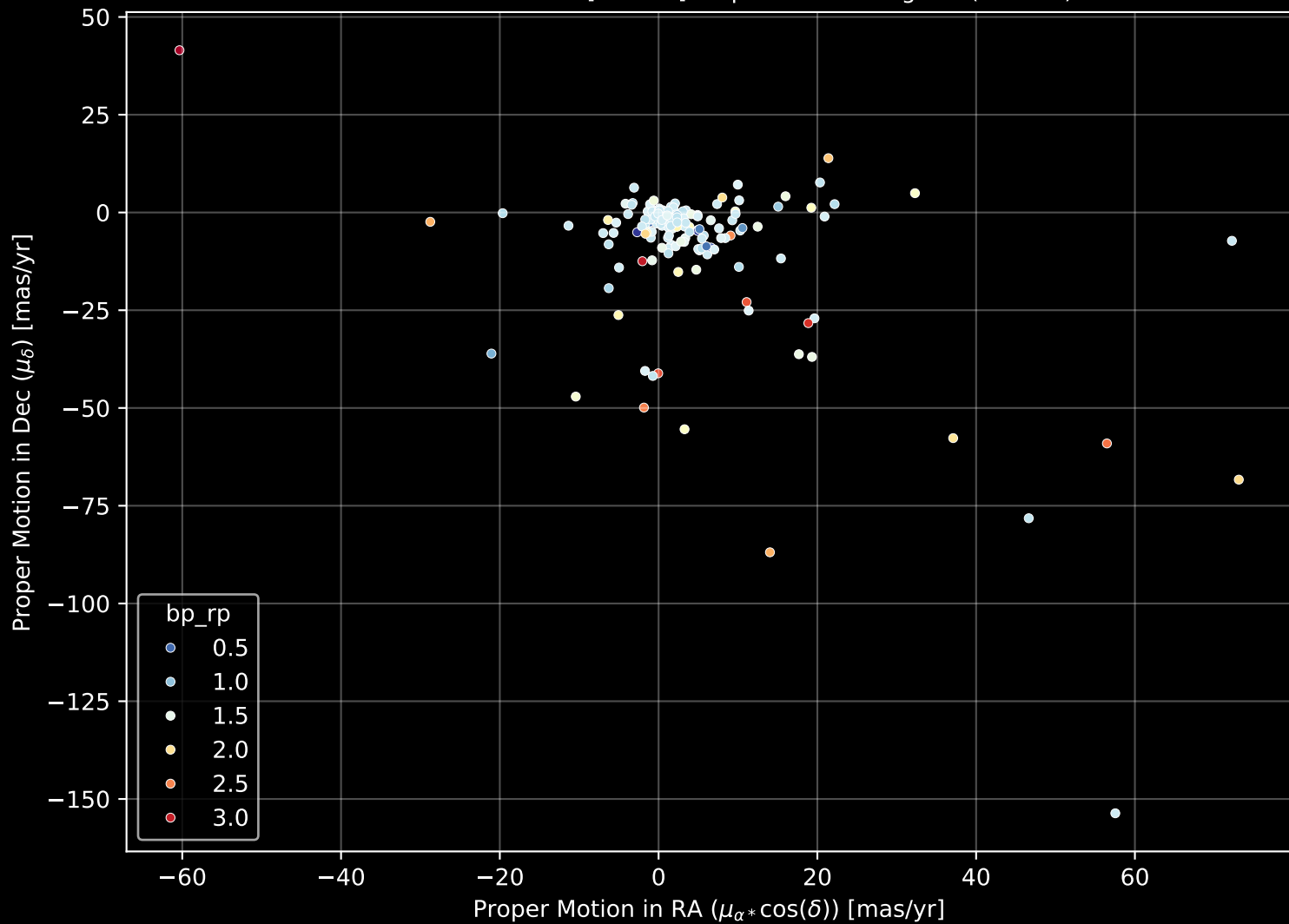
APOGEE DR17 Field: [190-19] Proper Motion Diagram (n= 179)
