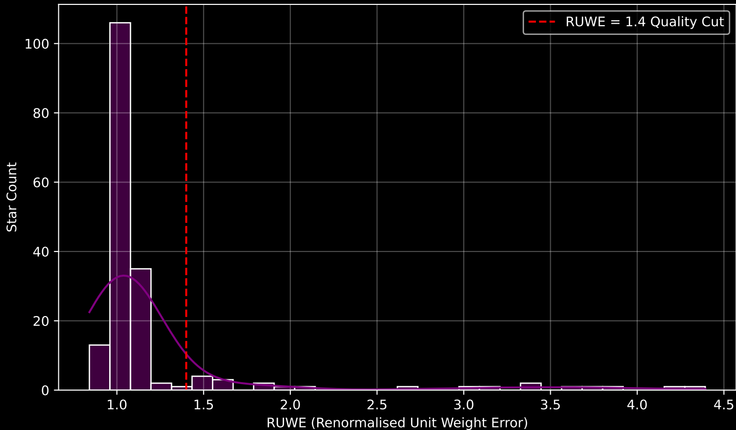
GAPOGEE DR17 Field [190-19] RUWE Distribution (n= 178)
