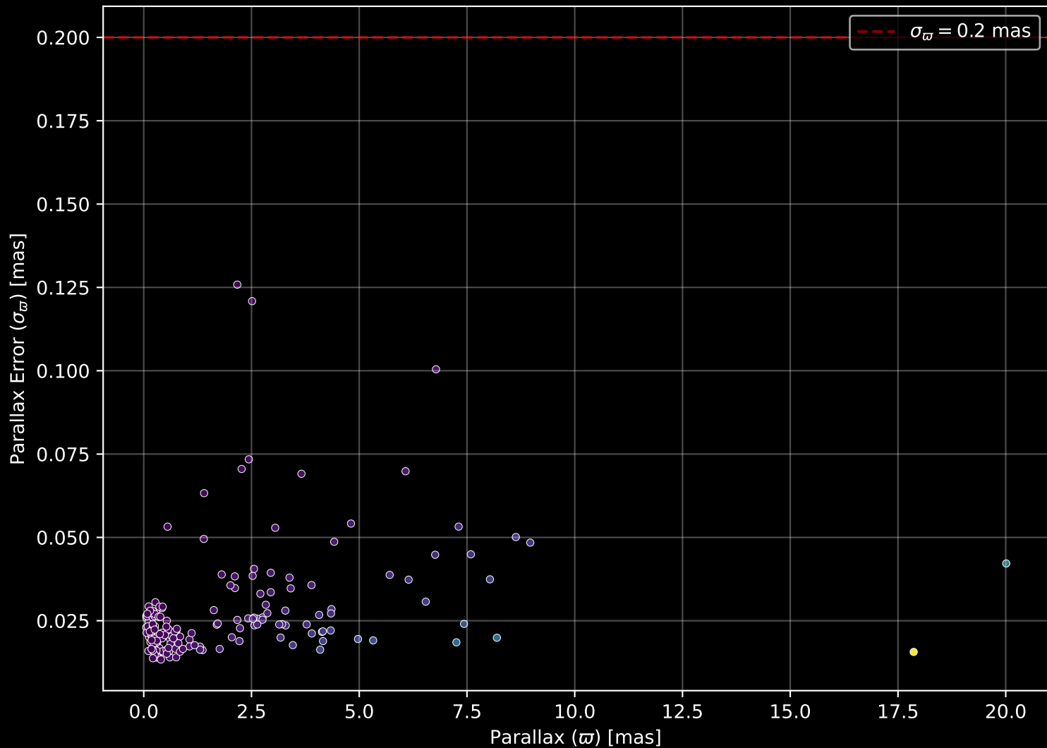
APOGEE DR17 Field: [190-19] Parallax Quality (n= 179)
