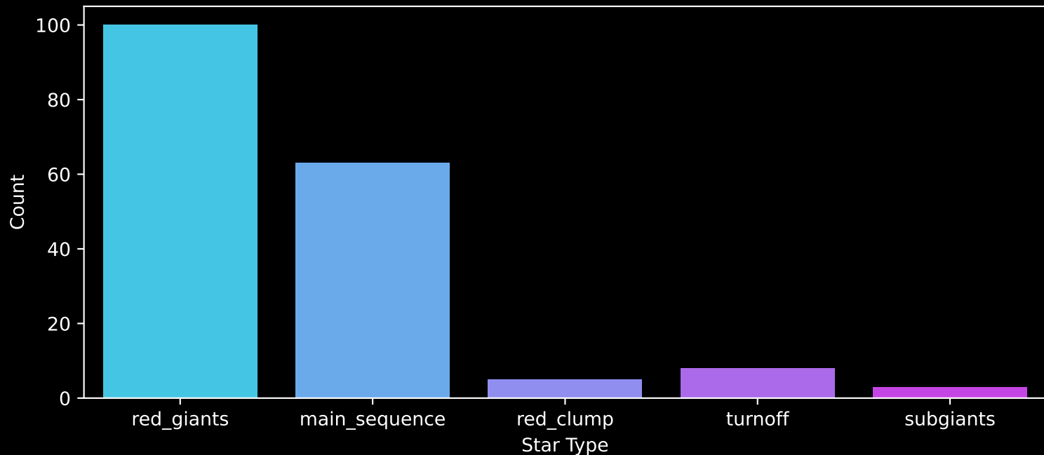
APOGEE DR17 Field: [190-19] Count plot of Star Type
