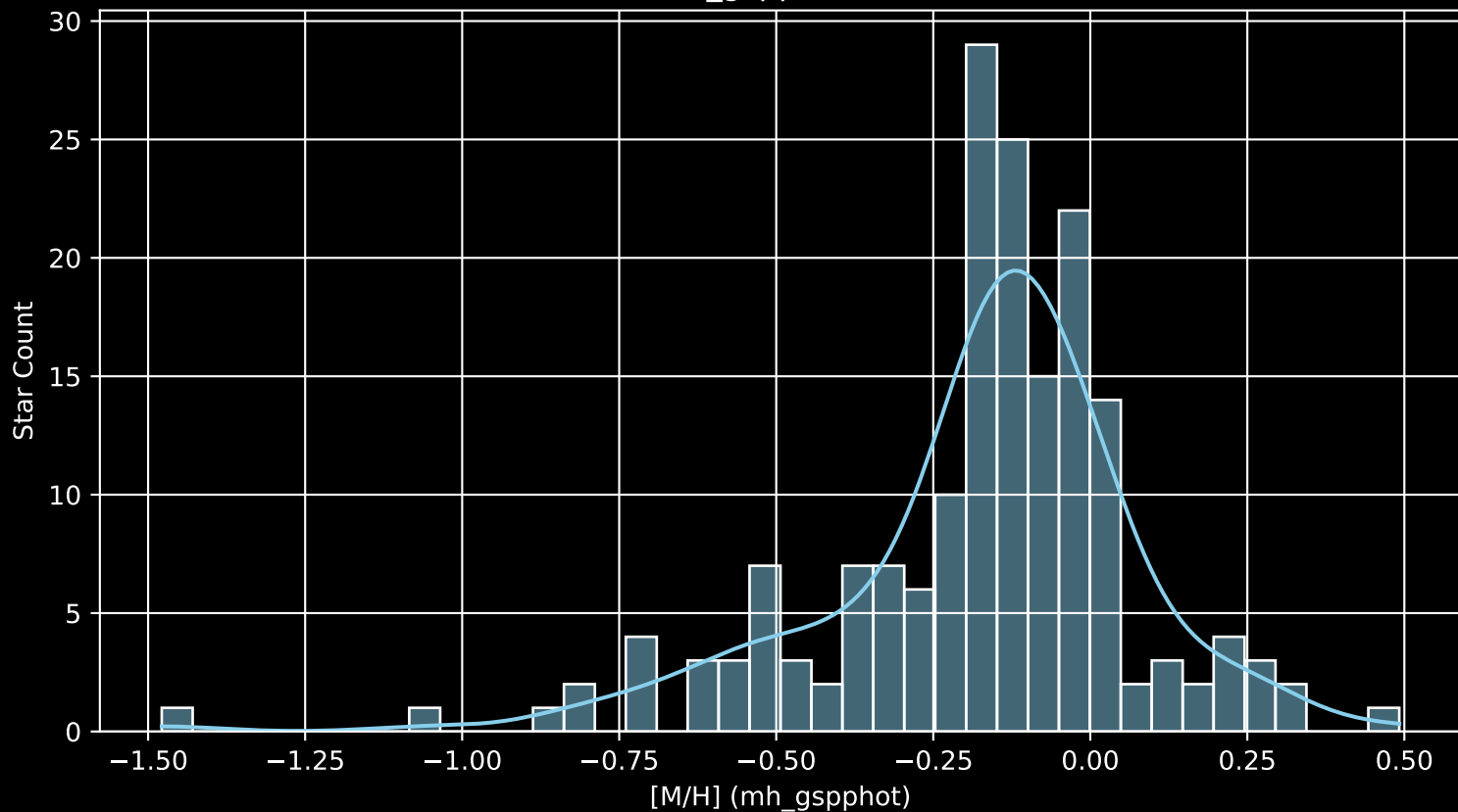
APOGEE DR17 Field: [190-19 [M/H] (mh_gspphot) (n= 179)
