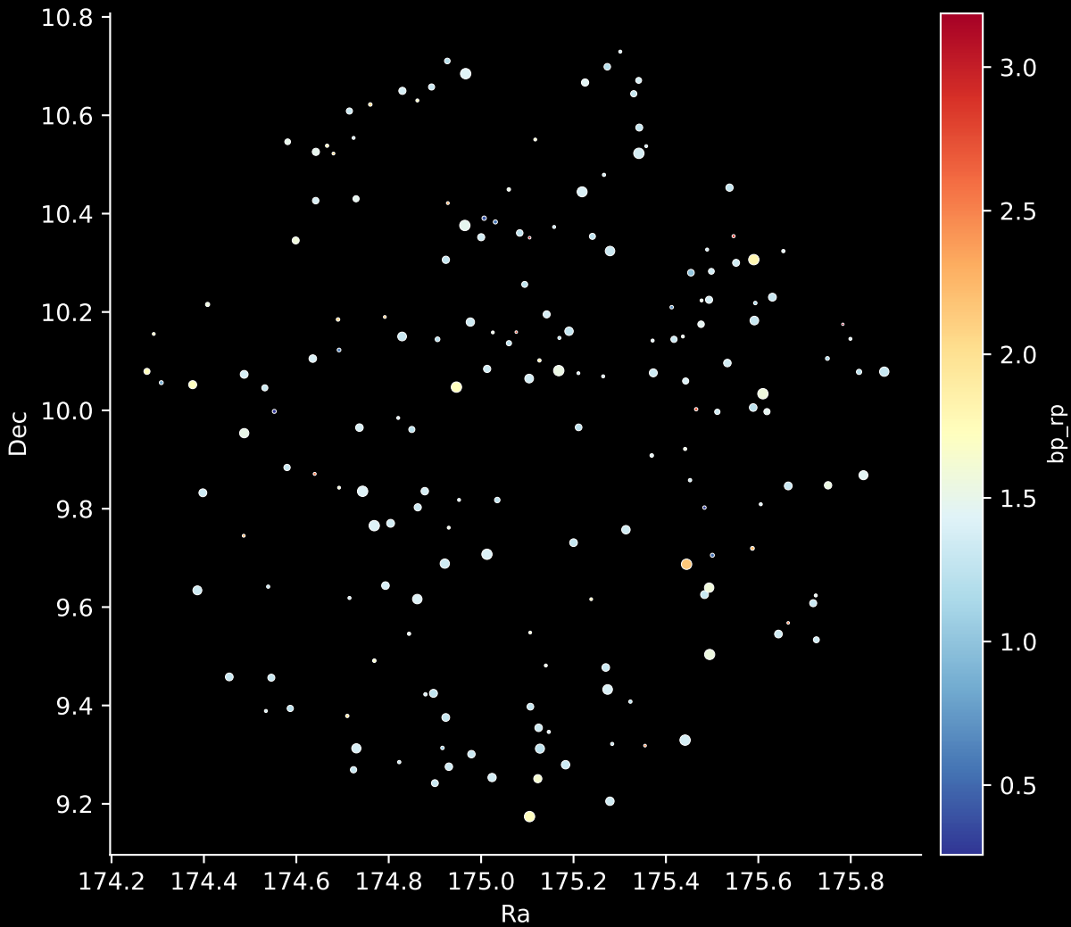
APOGEE DR17 Field: [190-19] Stars: 179
